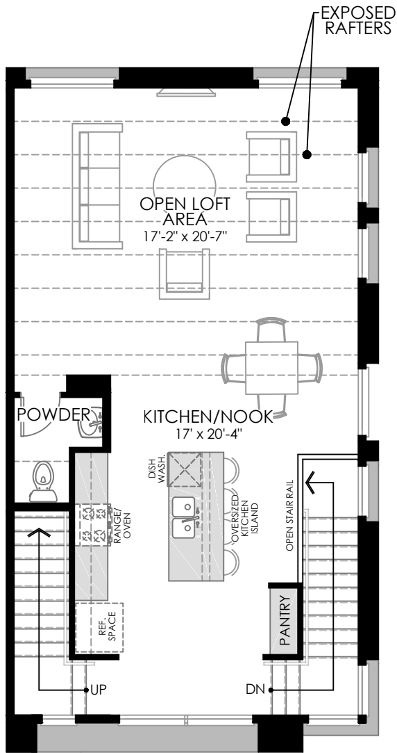
2 ND FLOOR
