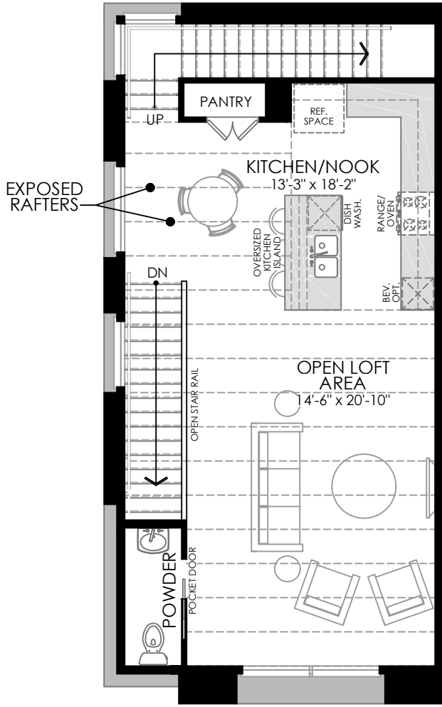
2 ND FLOOR
